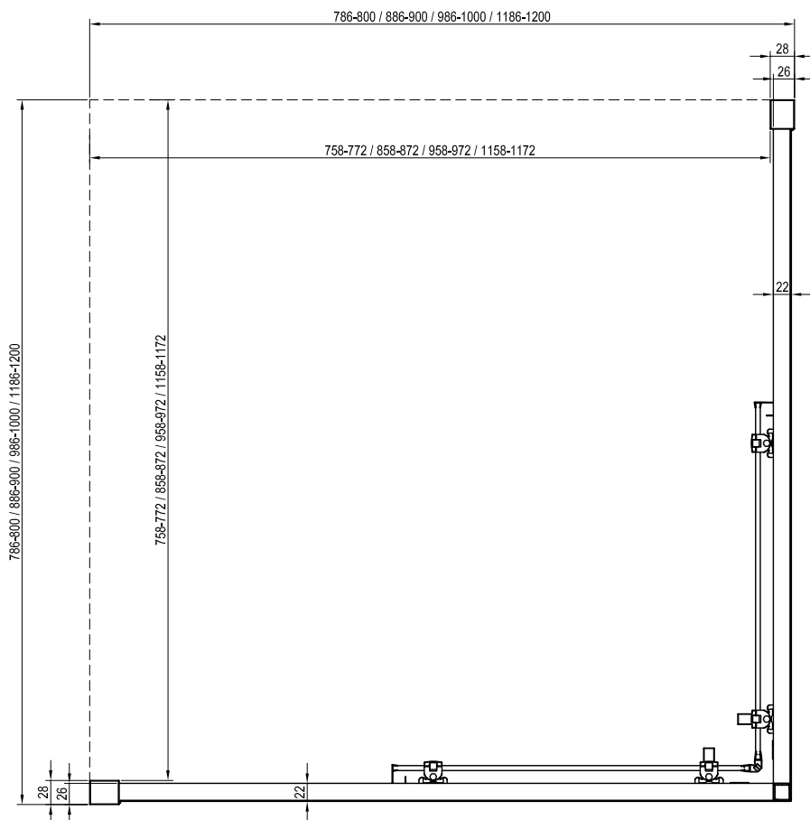
Technical drawing of shower enclosures BLSRV2 and BLSRV2K+BLSRV2K.
