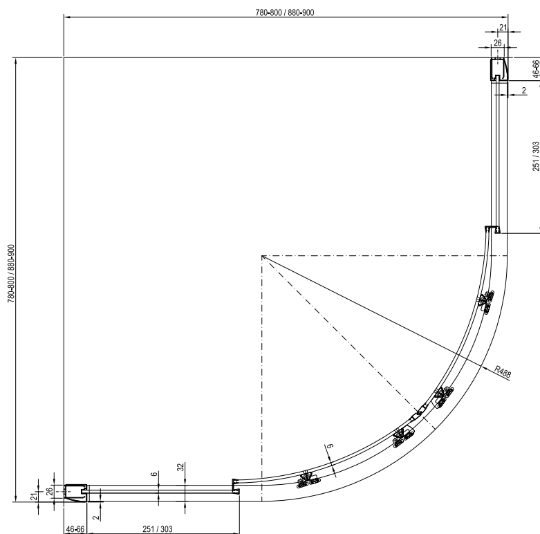
Technical drawing of shower enclosures BLCP4 and BLCP4 Sabina.
