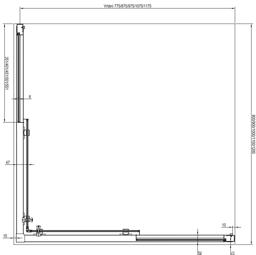
Technical drawing of shower enclosures NBLRV2 and NBLRV2K+NBLRV2K.
