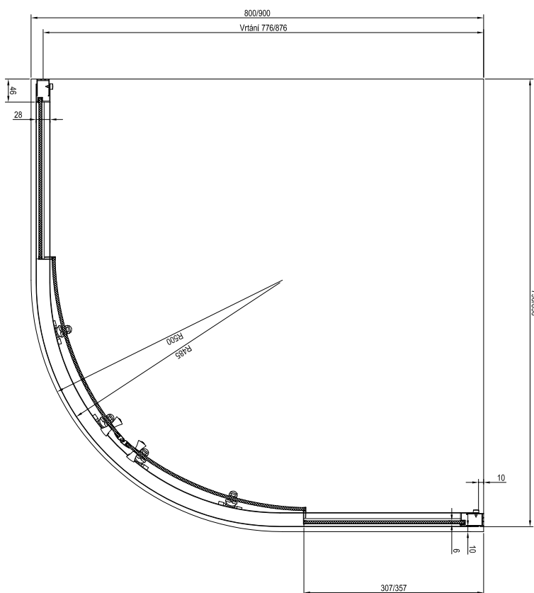
Technical drawing of shower enclosures NBLCP4 and NBLCP4 Sabina.
