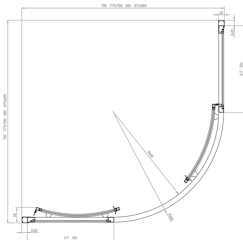
Technical drawing of shower enclosures SKCP4 and SKCP4 Sabina.
