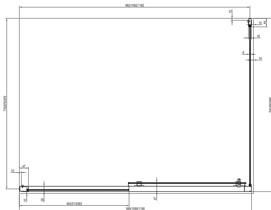
Technical drawing of shower door NBLDP2 and fixed wall NBLPS
