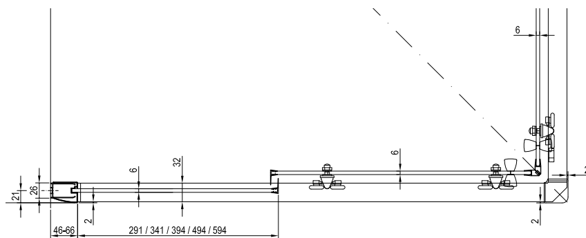
Technical drawing of shower enclosures BLRV2 and BLRV2K+BLRV2K.
