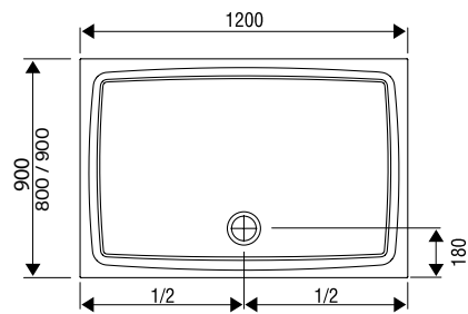
Gigant Pro 90x120
